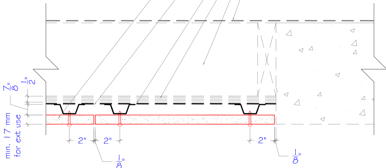
TYPICAL WALL SECTION - CONCRETE WALL INTERSECTION PLAN VIEW
