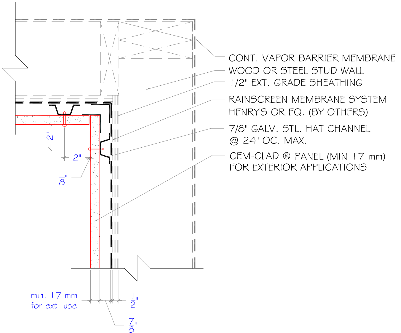
TYPICAL INSIDE CORNER
